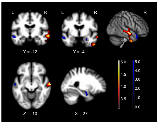
Fig. 2. T -score maps of brain areas for which smaller volume is associated with higher emotional contagion (IRI Personal Distress subscale score) when controlling for age, education, sex, diagnosis, field strength, and total intracranial volume ( n = 237 ). Smaller volume in right inferior, middle temporal, and superior temporal gyri was associated with higher emotional contagion after correction for type 1 error ( P_{FWE} < 0.05 ). At less stringent statistical thresholds, smaller volume in left middle temporal gyrus, right temporal pole, right anterior hippocampus, and right parahippocampal gyrus were also associated with higher emotional contagion ( P < 0.001 , uncorrected). Color bars represent T scores (hot, P_{FWE} < 0.05 according to study-specific permutation analysis; blue, P < 0.001 , uncorrected; T > 3.13 and cluster size > 150 \text{ mm}^3 ). Results are overlaid on a DARTEL-derived template of 50 older healthy controls.
