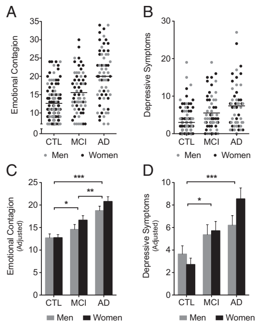
Fig. 1. Emotional contagion and depressive symptoms in MCI and AD are higher than in healthy controls (CTL). (A) Raw emotional contagion (IRI Personal Distress subscale) and (B) depressive symptom (GDS) scores for the CTL ( n = 111 ), MCI ( n = 62 ), and AD ( n = 64 ) groups. Kolmogorov-Smirnov tests of normality indicated that there was a normal distribution of emotional contagion scores in MCI ( P > 0.05 ) and AD ( P > 0.05 ). (C) Emotional contagion and (D) depressive symptoms, adjusted for age and education and stratified by sex, were higher in patients than in healthy controls. Significant main effects of diagnosis are denoted by * P < 0.01 , ** P < 0.001 , and *** P < 0.0001 . Error bars represent SEMs.
